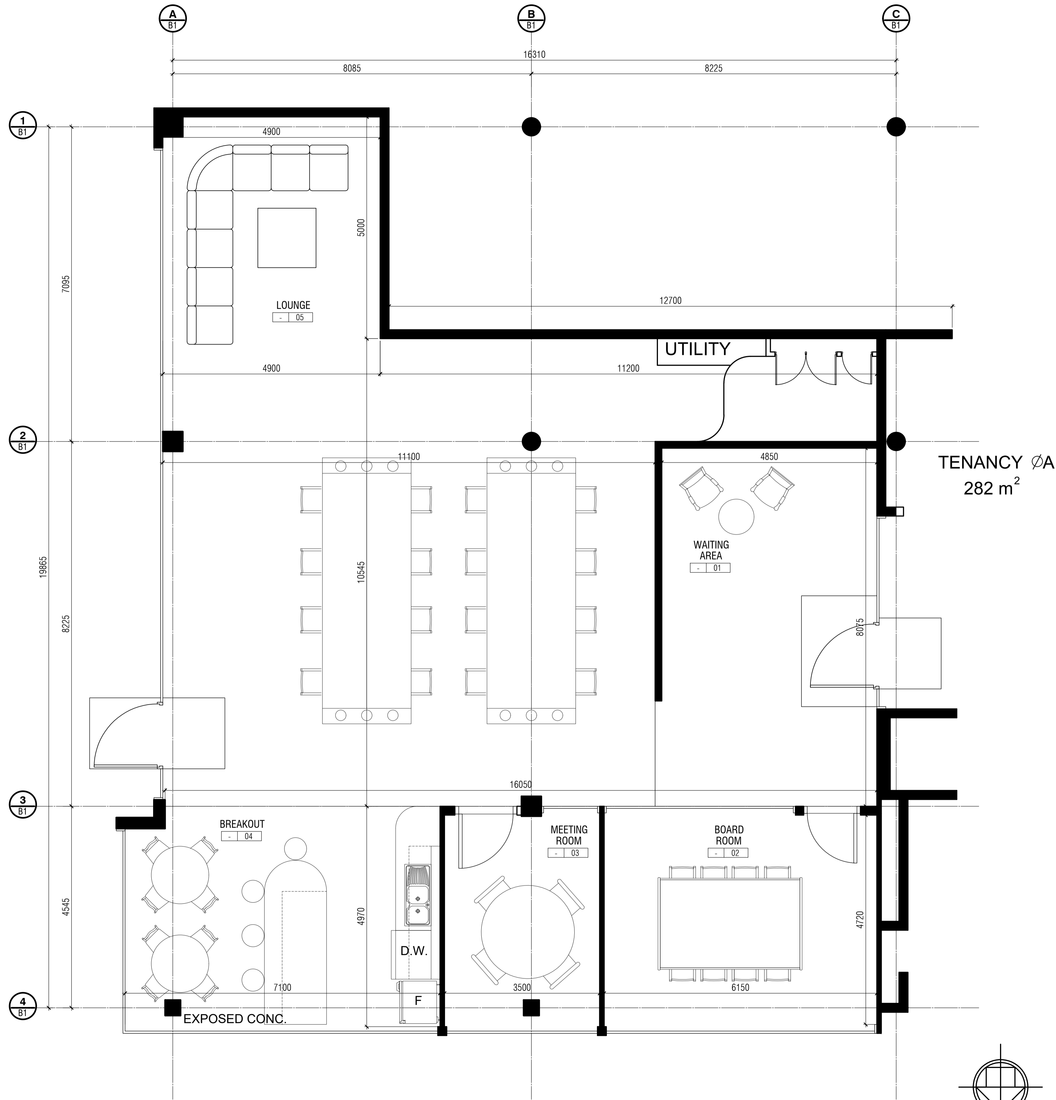
FLOOR PLAN SCALE 1:50
